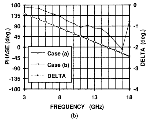
Fig. 5. Standard coaxial short circuit reflection coefficient measured at port 2 [case (a)] and port 3 [case (b)]. Since the phase plots are quite similar, their difference DELTA is also plotted in figure 5(b).
