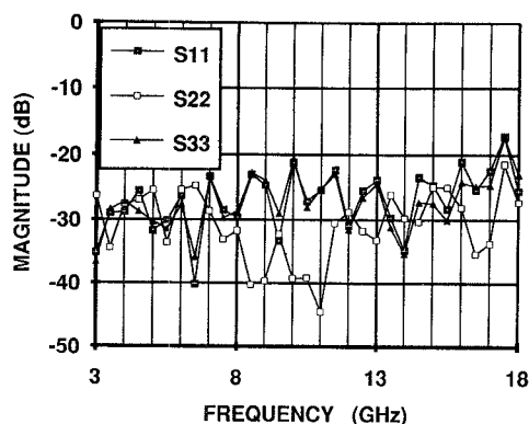
Fig. 9. Directional coupler S_{ii} parameters magnitude.
