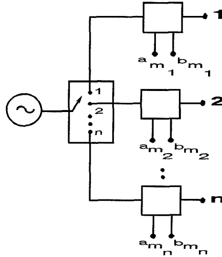
Fig. 2. Generalized model of a multiport test set.
